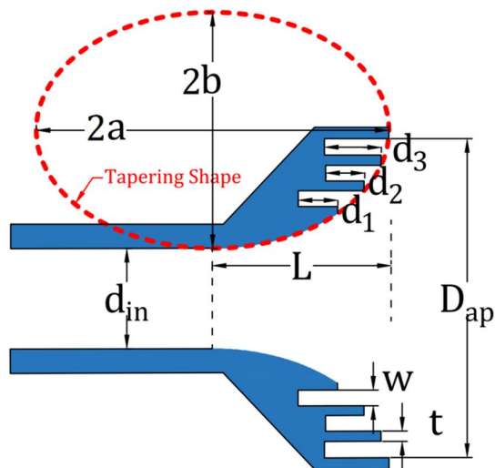
Figure 4: Side view of axially corrugated horn antenna with the proposed aperture taper based on an elliptical function.
