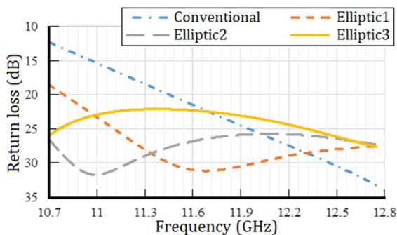
Figure 5: Comparison of the return loss of the proposed antenna with the conventional axial corrugated horn antenna.
