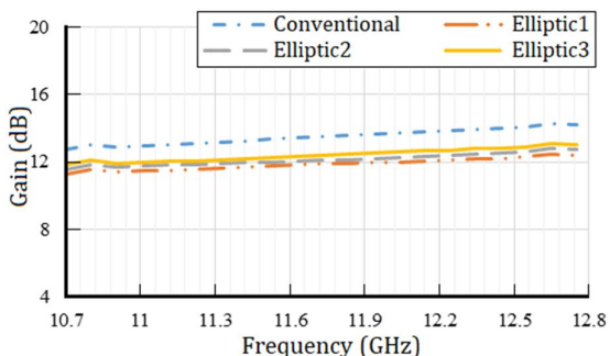
Figure 6: Comparison of the gain of the proposed antenna with the conventional axial corrugated horn antennas.
