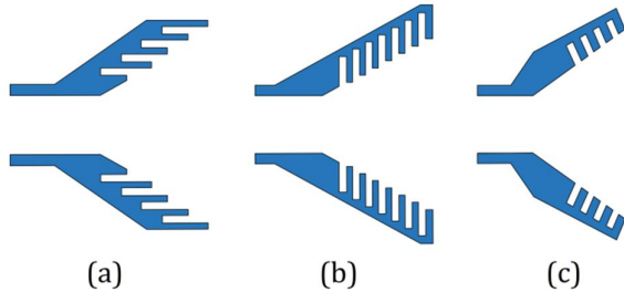
Figure 2: Common types of grooves in corrugated horn antenna. (a) Axial corrugation, (b) Scalar corrugation, (c) Standard (normal) corrugation.
