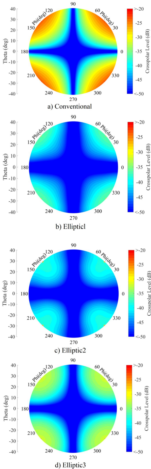
Figure 8: The cross-polar level versus Theta and Phi angles at 11.7 GHz. a) Conventional antenna, b) Proposed elliptical1 antenna, c) Proposed elliptical2 antenna and d) Proposed elliptical3 antenna.
