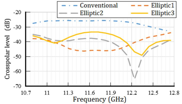
Figure 7: Comparison of the cross-polar levels of the proposed antenna with the conventional axial corrugated horn antennas at 70^\circ beamwidth.
