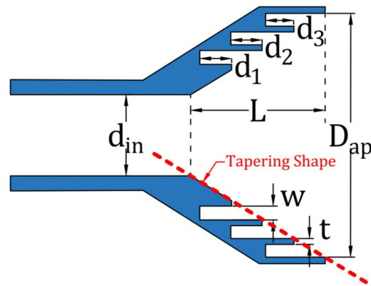
Figure 3: Side view of a conventional axially corrugated horn antenna.
