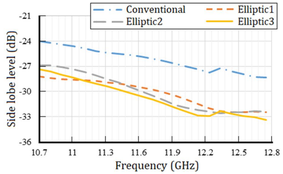
Figure 9: Comparison of the side-lobe levels of the proposed antenna with the conventional axial corrugated horn antenna.
