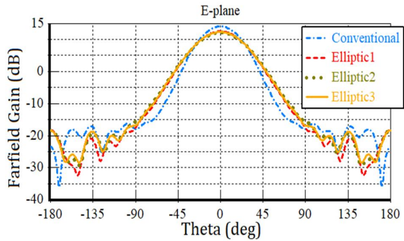
Figure 10: Optimized E-plane far-field radiation patterns for the proposed and the conventional axial corrugated horn antennas.
