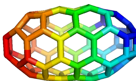
Figure 3. The Case of n = 4 in C_{16n+4} .
