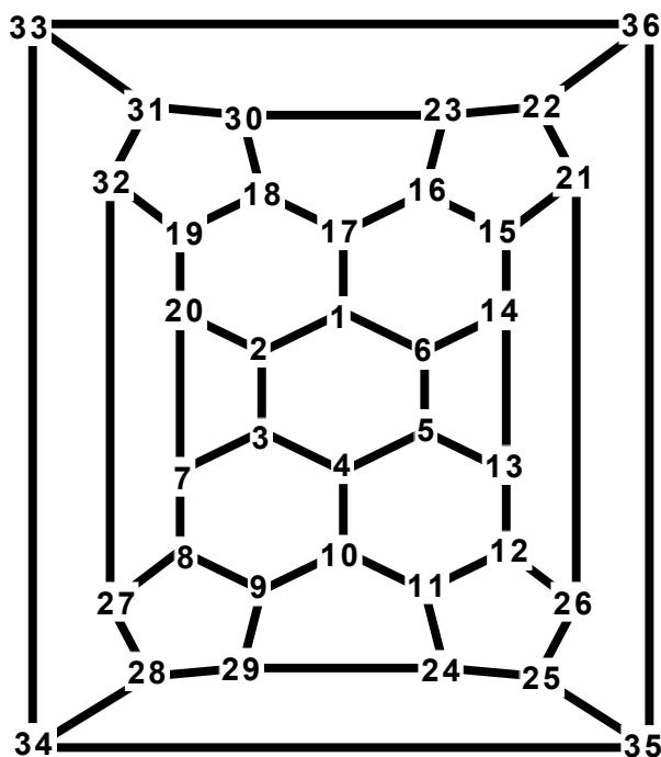
Figure 1. Labeling of fullerene C_{16n+4} for n=2 .
