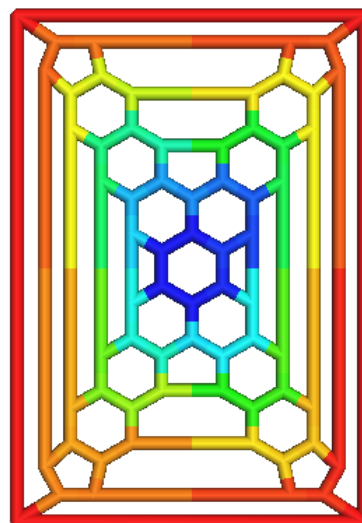
2-D graph of C_{16n+4} for n = 4 .
