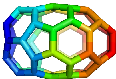
Figure 2. The Case of n = 3 in C_{16n+4} .
