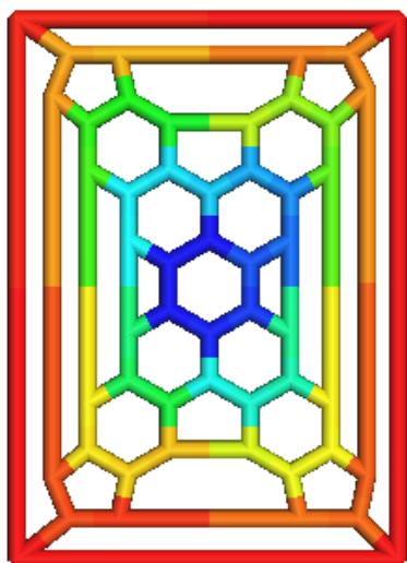
2-D graph of C_{16n+4} for n = 3 .
