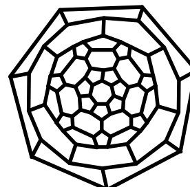
A fulleren with 16 hexagons.
