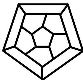
A fulleren without hexagons
