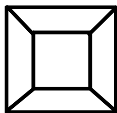
A fulleren without hexagons
