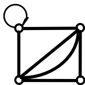
Figure 1. A graph with a loop and two parallel edges.
