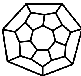
A fulleren with 2 hexagons.
