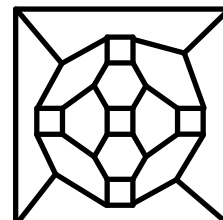
A fulleren with 12 hexagons.
