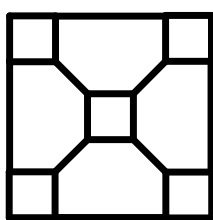
A fulleren with 4 hexagons.
