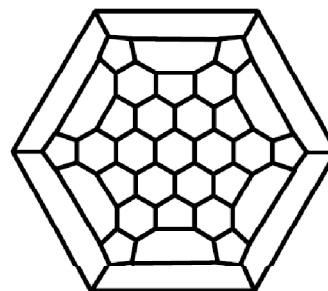
A fulleren with 26 hexagons.
